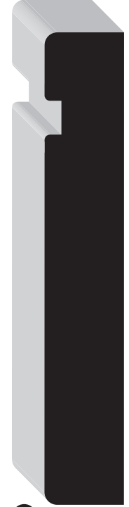
M 09091 5/8" x 3-1/2" PMDF 16'
