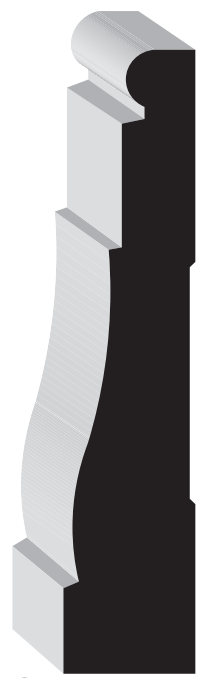
OW445 WM445 11/16" x 3-1/4" PFJP • SO 15' • RL
